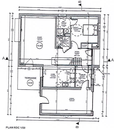
PLAN RDC 1/50
